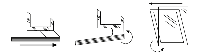
Figure 2: Movement from thermal expansion and contraction and/or glass rotation
